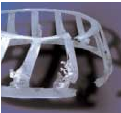
Cage damage due to incipient seizing
